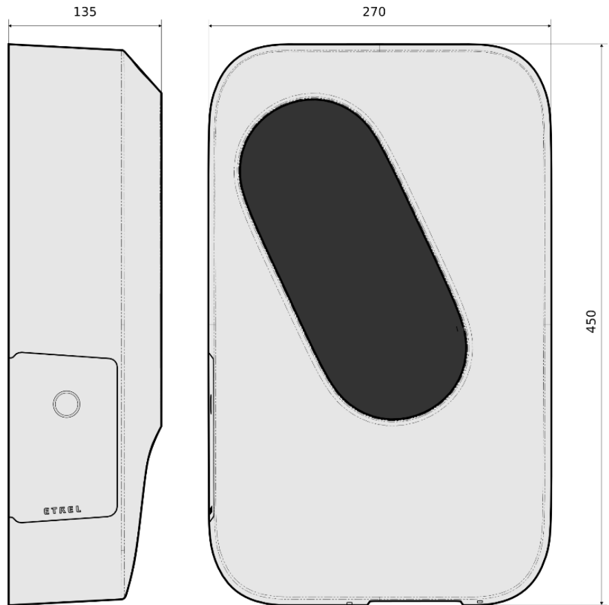
Figure 5: Dimensions of the charging station
